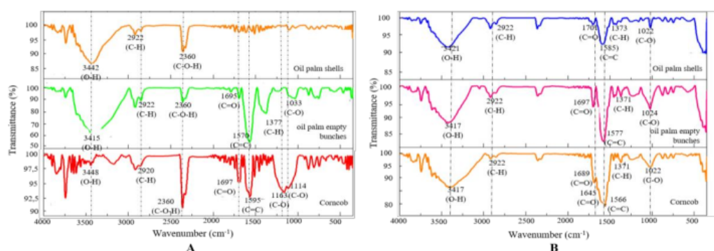
Fig. 1. A. FTIR spectrum of biochar surface functional groups of (oil palm shells, oil palm empty fruit bunches, corncoobs) at 4 pyrolysis temperatures of 300-400°C. B. FTIR spectrum of biochar surface functional groups (oil palm shells, palm oil palm bunches and corncoobs) after inoculated with alginate-producing bacteria (KK1-40) incubation for 28 days at 28°C
