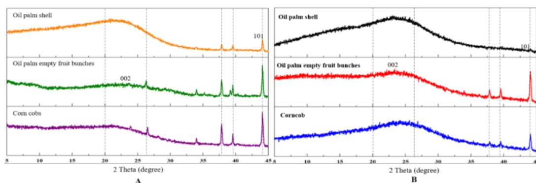
Fig. 2. A. XRD spectrum of biochar structures (oil palm shells, oil palm empty fruit bunches, corncobs) at pyrolysis temperatures of 300-400°C, B. XRD spectrum of biochar structures (oil palm shells, palm oil palm bunches and corncobs) following inoculation with alginate-producing bacterial isolates for 28 days at 28°C
